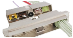
SIM/EN4165 series 2 connectors
