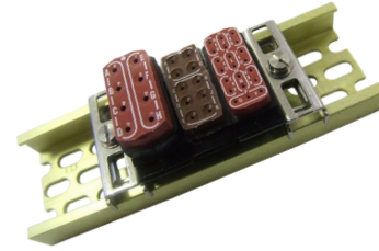
1100 modules + metallic rail
