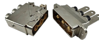
H-PAC connectors
