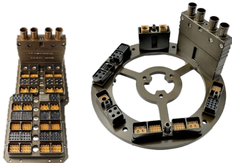
SIM/EN4165 metallic plates
