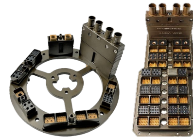
SIM/EN4165 metallic plates
