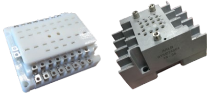
Relay sockets for signaling with integrated PCB for distribution
