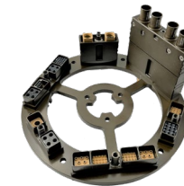
SIM/EN4165 metallic plates
