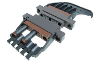
1900/EN3545 connectors
