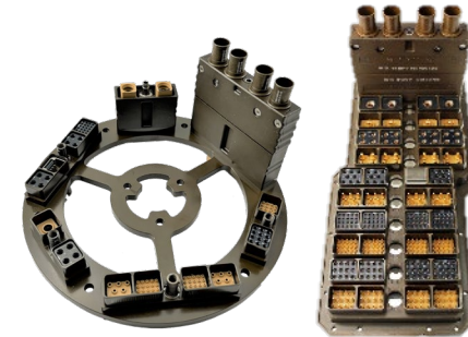
SIM/EN4165 metallic plates
