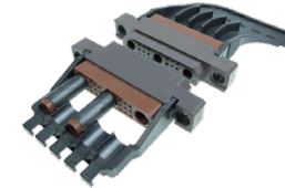
1900/EN3545 connectors
