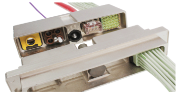
SIM/EN4165 connectors - series 2
