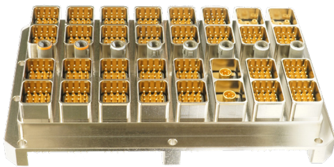
SIM / EN4165 metallic plates (example with SIM modules equipped with standardized crimp contacts with gold protection)
