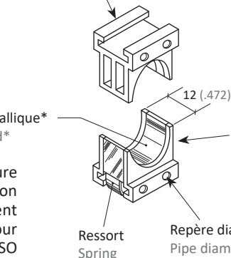
3.1 Demi bride conductrice Conducting half clamp
