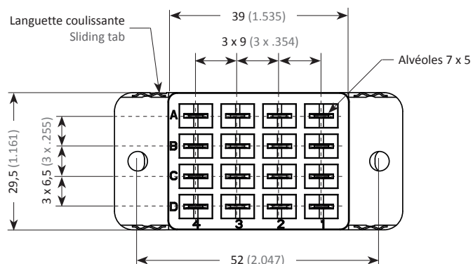
Socle de relais 4RT bistable Bistable 4RT relay socket
